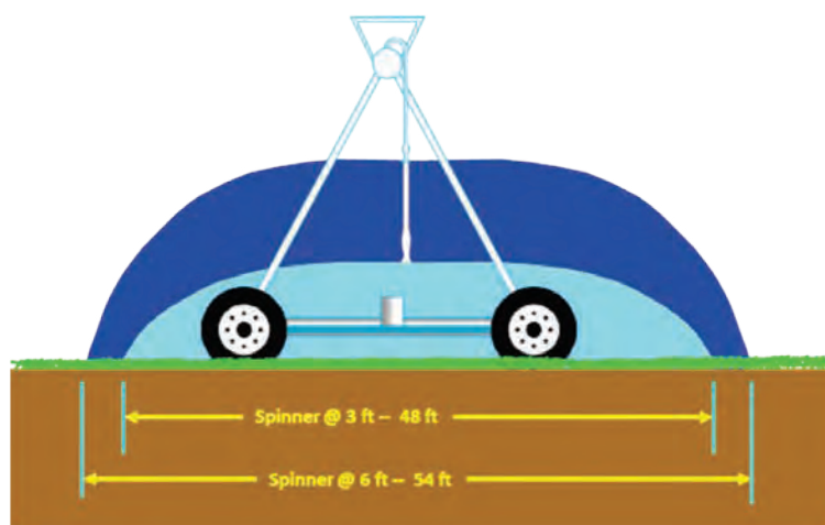
Figure L-4. Examples of the wetted diameter for Spinner devices from the Nelson Irrigation Corporation.
