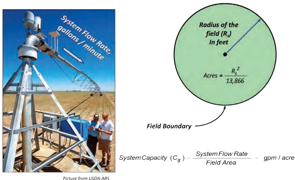
Figure L-2. Definition of system capacity for a field irrigated by a center pivot.
