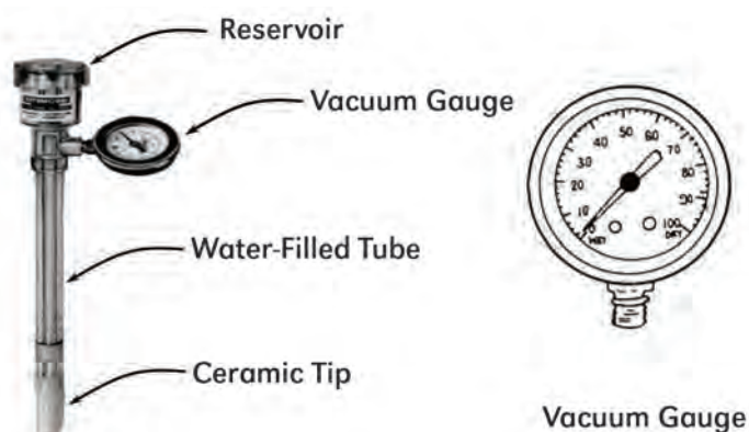
Figure J-5. Components of tensiometers used to measure soil matric potential.
