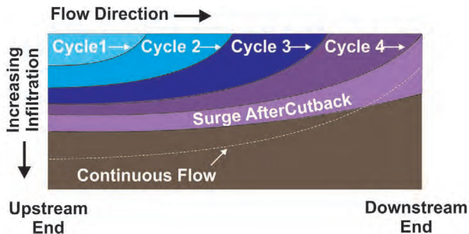
Figure K-7. Comparison of infiltration profiles for surge and continuous flow furrow irrigation systems.
