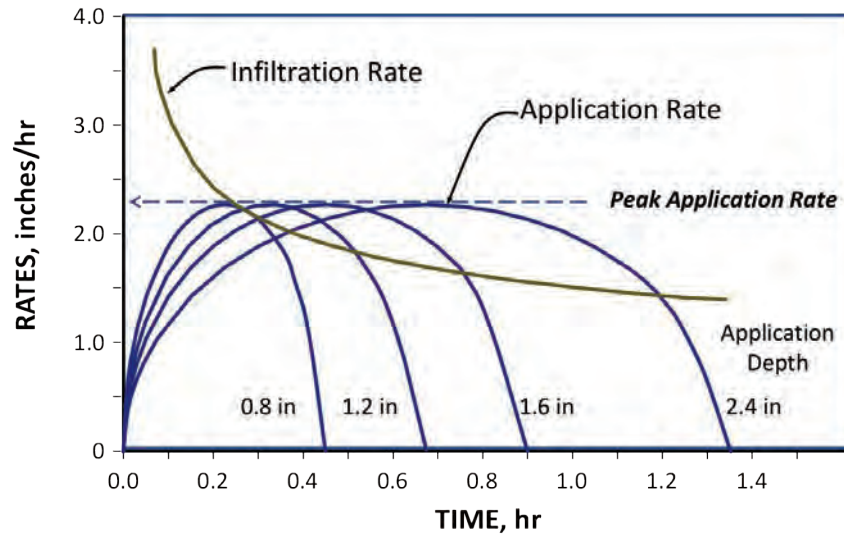
Figure L-7. Effect of water application depth per irrigation on runoff potential.
