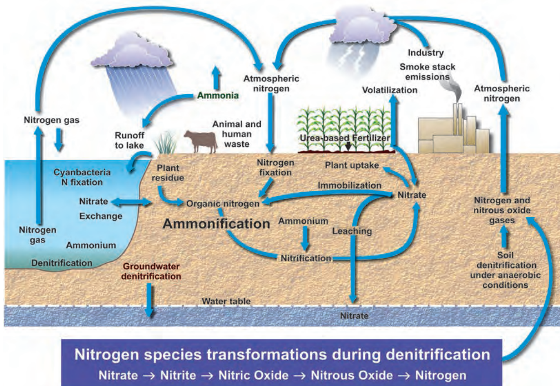
Figure D-1. Generalized nitrogen cycle within water, soil and in the air.
