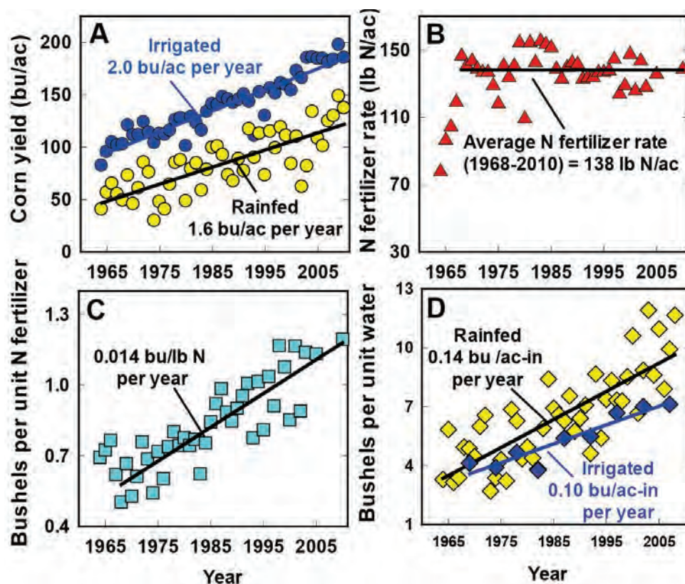
Figure B-2. Trends in corn grain yield (A), N fertilizer rate (B), grain yield produced per unit of N fertilizer ( NUE_f ) (C), and per unit of in-season water (WUE) (D) for the period from 1965-2010. Separate trends are shown for rainfed (yellow) and irrigated crops (blue) in (A) and (D). In-season (May-Aug.) water includes rainfall and irrigation. Rainfall data (D) were retrieved from five representative locations in Nebraska. Yield, N fertilizer, and irrigation water data were retrieved from USDA-NASS.
