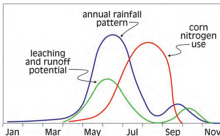
Figure G-2. Depiction of typical nitrogen uptake and the potential for nitrate leaching and runoff caused by precipitation during the growing season.
