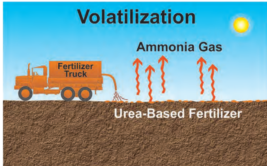
Figure D-6. Volatilization occurs when manures or ammonia containing fertilizers are on the soil surface.
