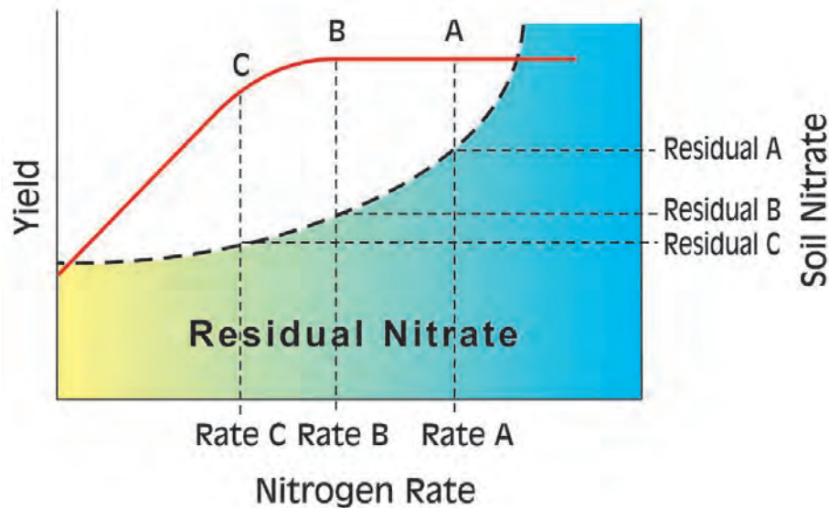
Figure G-3. Impact of excessive nitrogen application rate on soil residual nitrogen.
