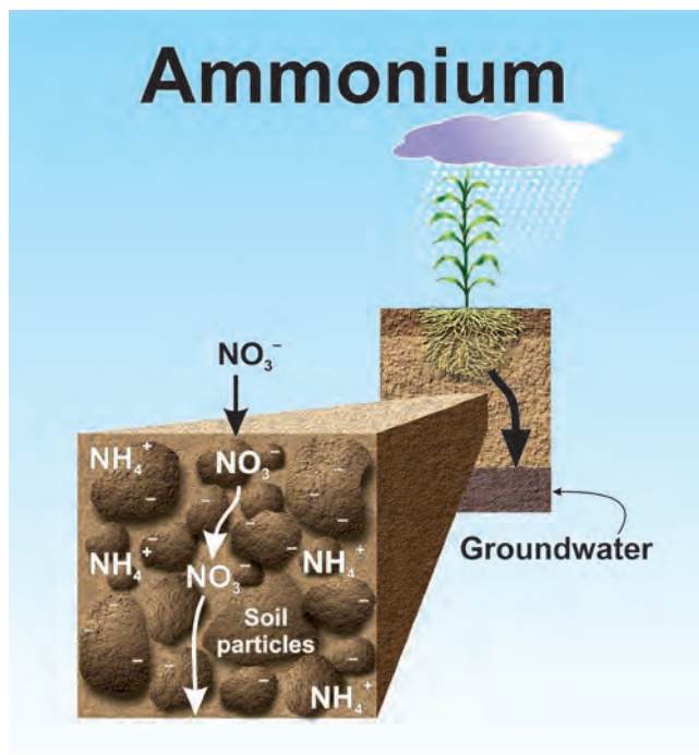
Figure G-5. Depiction of the attachment of positively charged ammonium molecules to negatively charged soil particles, which prevents leaching of N in the ammonium form while allowing leaching in the nitrate form.
