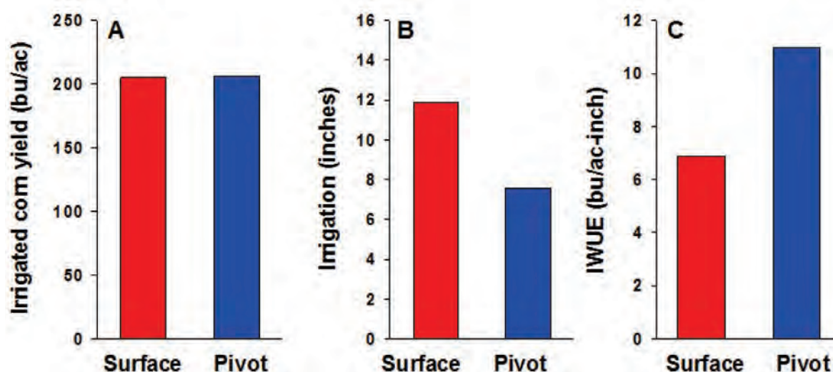
Figure B-6. Average (2006-2011) irrigated yield (A), irrigation inches applied (B), and irrigation water use efficiency (IWUE) (C) in surface- and pivot-irrigated corn fields in the South Central region.
