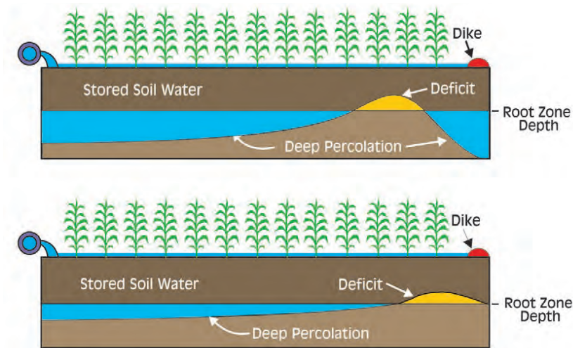
Figure K-3. Infiltration profiles under conventional furrow irrigation with blocked-end furrows (top) and three-quarter-plus advance rule (bottom).
