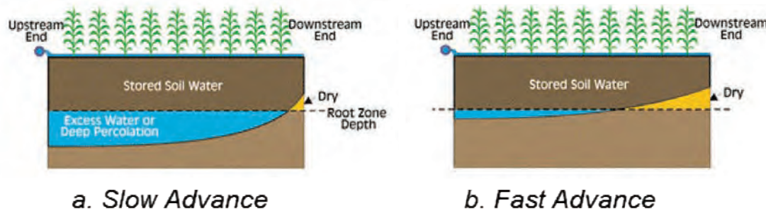
Figure K-2. Soil water infiltration pattern for furrow irrigated fields with slow (a) and fast advance (b) times.
