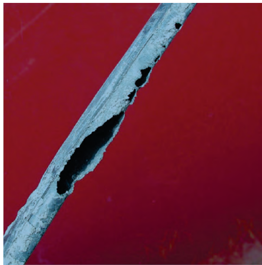
Figure M-5. Holes in SDI drip tape from rodent damage.
