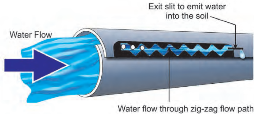
Figure M-2. Schematic drawing of a subsurface drip emitter.
