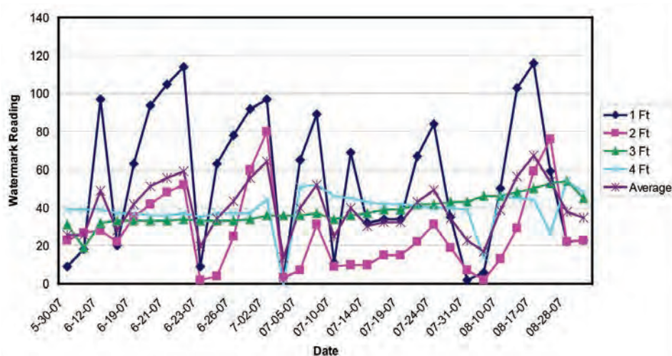
Figure J-7. Watermark record of one growing season.
