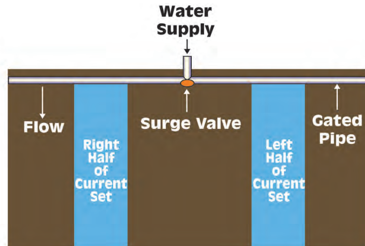
Figure K-6. Typical surge irrigation field layout.
