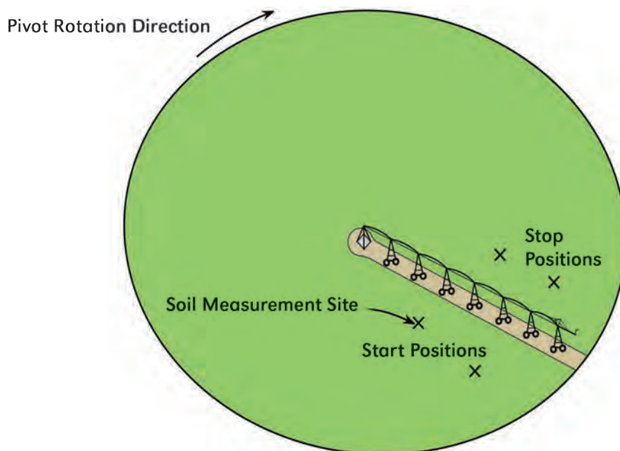
Figure J-9. Sensor placement at starting and stopping positions in a center-pivot irrigated field.
