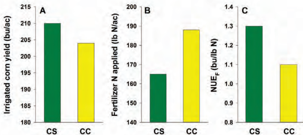
Figure B-5. Average (2006-2011) yield (A), fertilizer N (B), and fertilizer nitrogen use efficiency NUE_F (C) in irrigated corn grown in corn-soybean rotations (CS) versus continuous corn (CC) in the South Central region.
