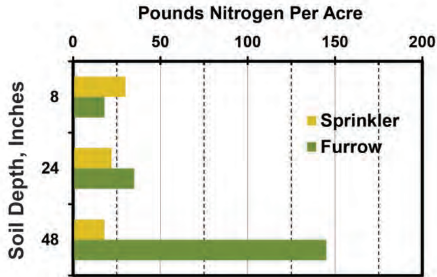
Figure E-1. Summary of two sets of soil samples: 1) taken from a soil that was sprinkler irrigated; and 2) taken from a soil that was irrigated by a furrow irrigation system.
