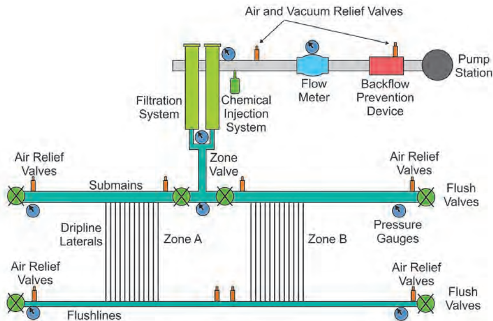
Figure M-3. Installation components recommended for an SDI system (modeled after image by Kansas State University).
