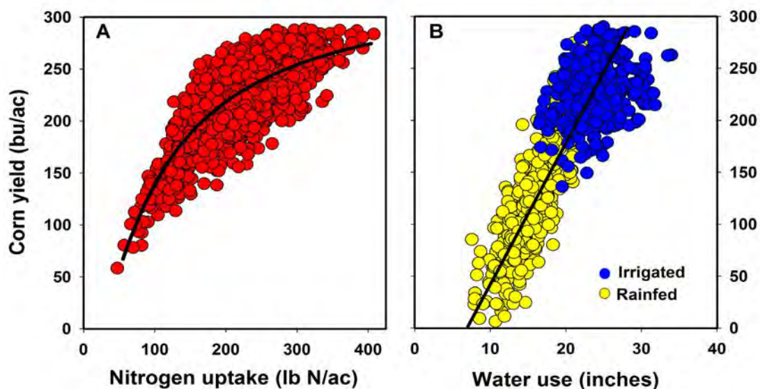
Figure B-1. Relationship between corn yield and corn N uptake (A) and corn yield and water use or crop ET (B). (Adapted from Grassini et al. 2009 and Setiyono et al. 2010).
