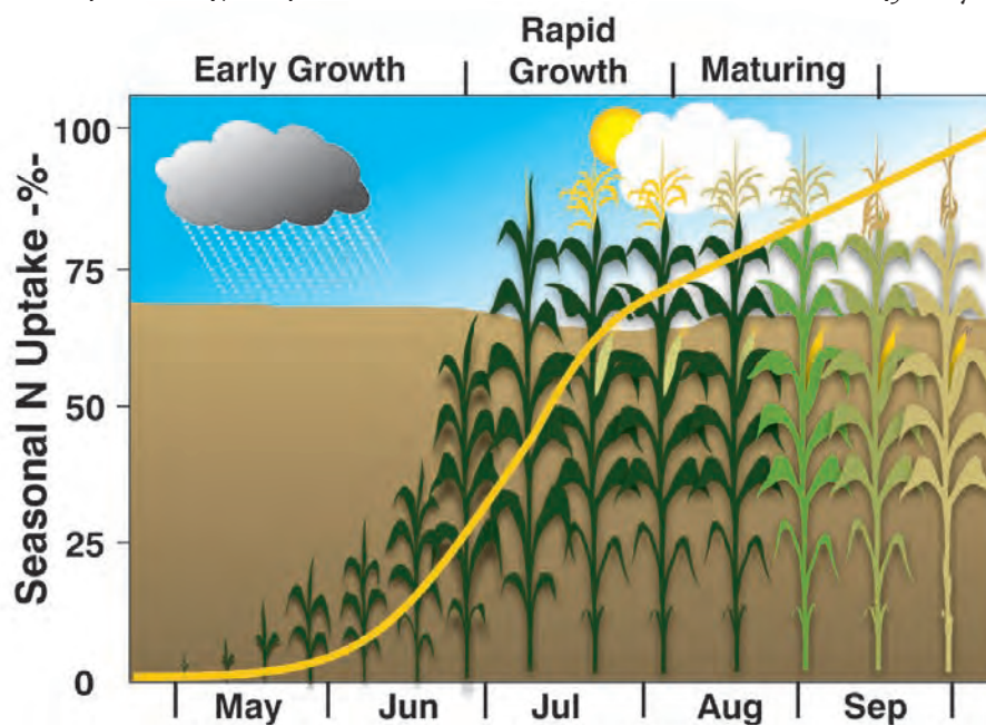
Figure G-1. Cumulative nitrogen uptake curve for a growing season.
