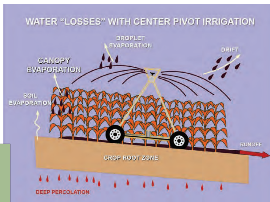
Figure J-1. Schematic drawing showing the major water losses that occur during a water application event using a center pivot irrigation system.
