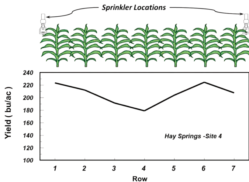
Figure L-5. Variation of yield for wide spacing of sprinklers perpendicular to rows of corn.
